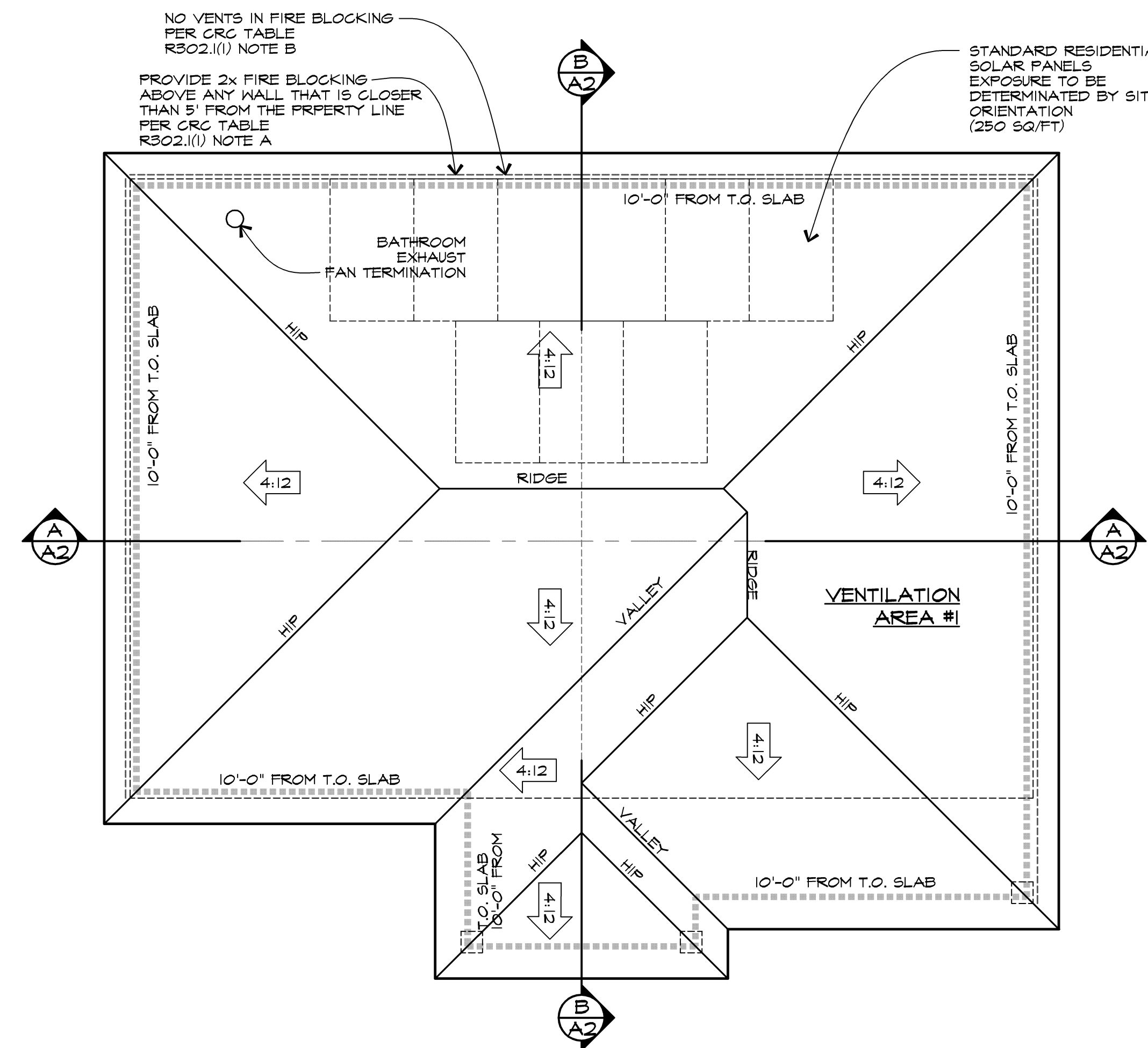
ROOF PLAN
