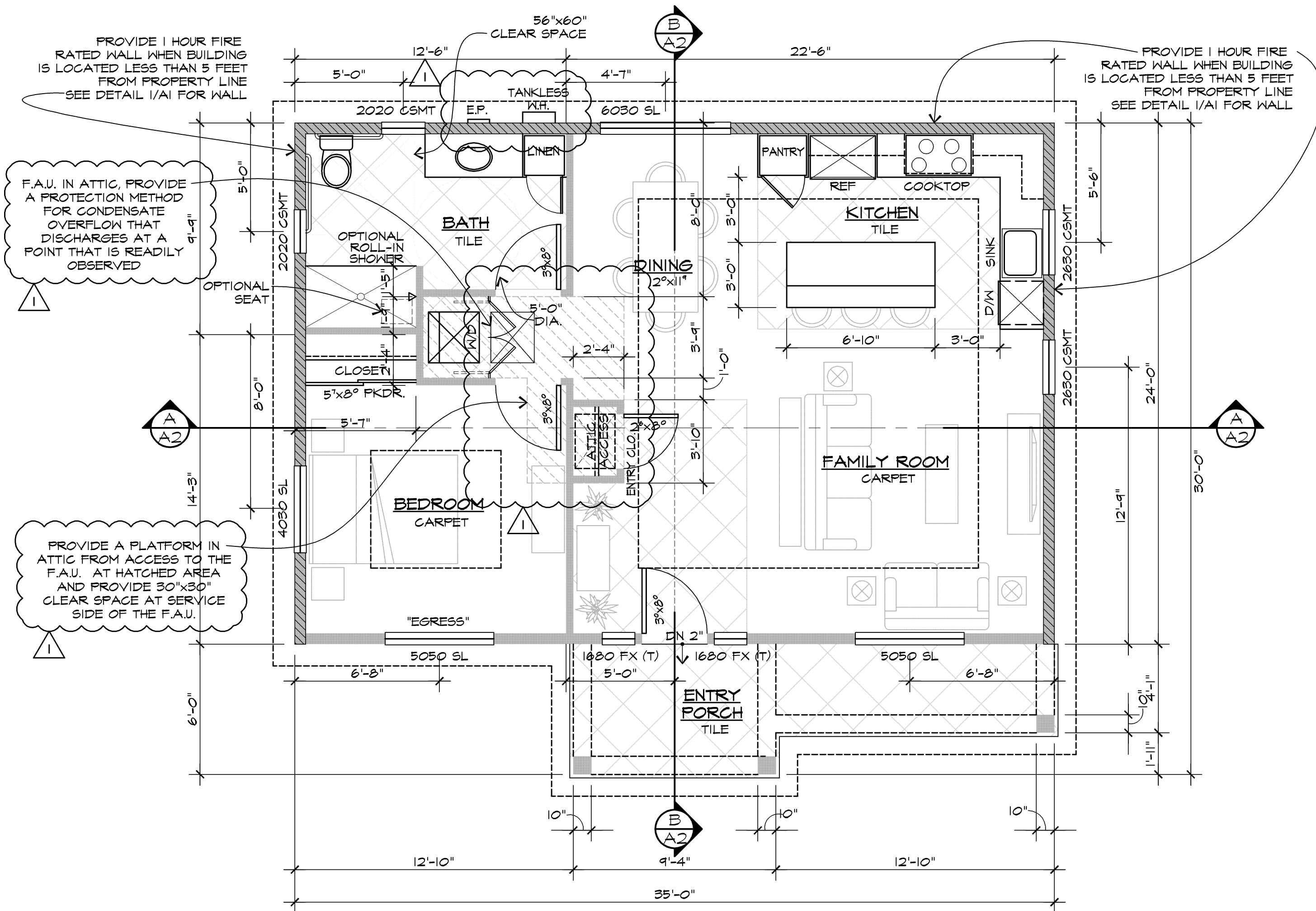
FLOOR PLAN (MEDITERRANEAN STYLE)
