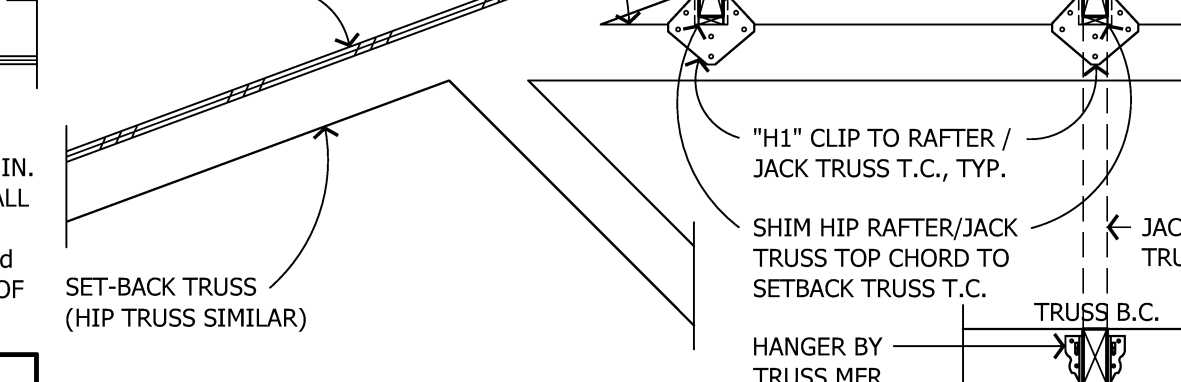
419 CONNECTION AT SET-BACK TRUSS
