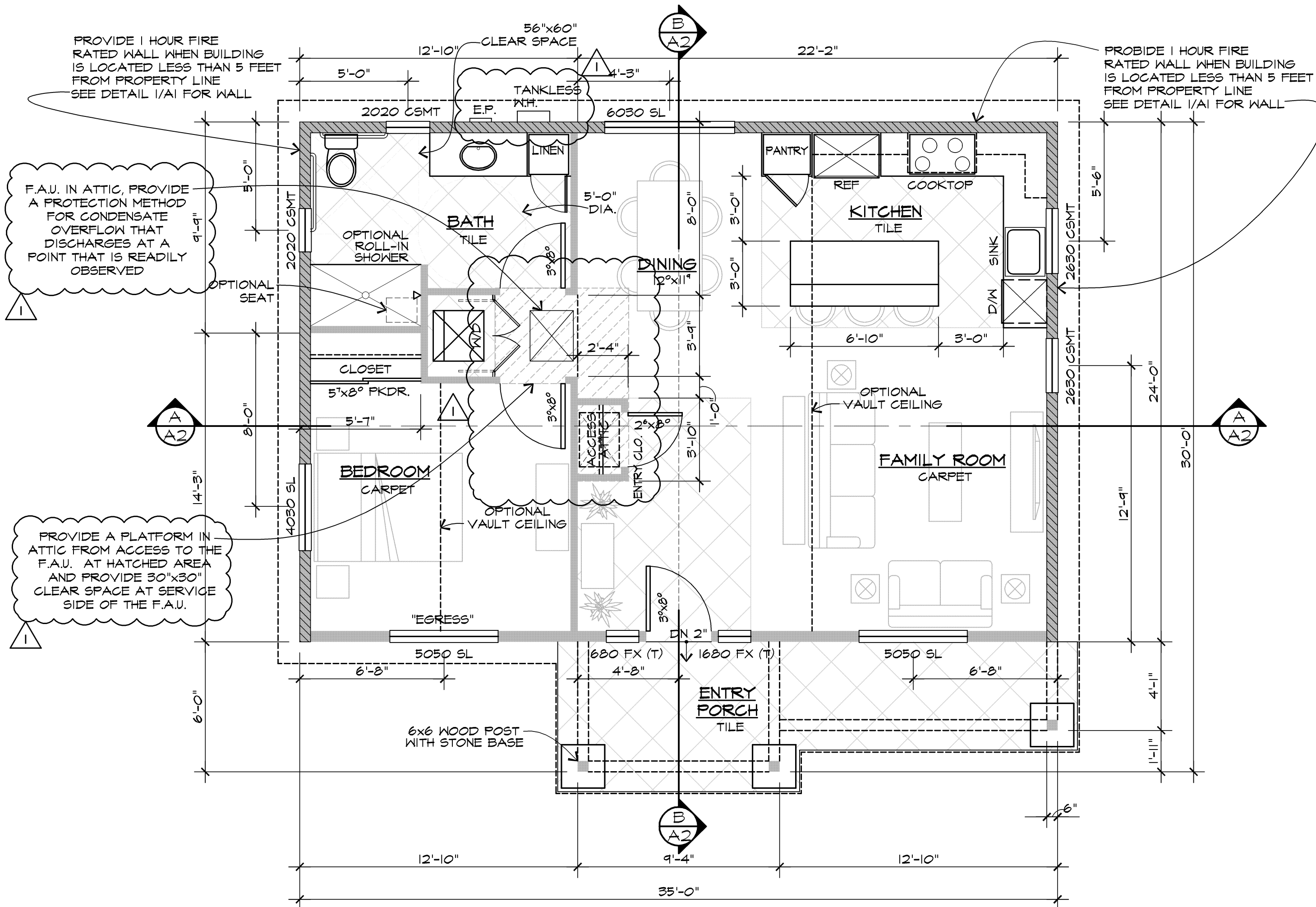
FLOOR PLAN (CRAFTSMAN STYLE)
