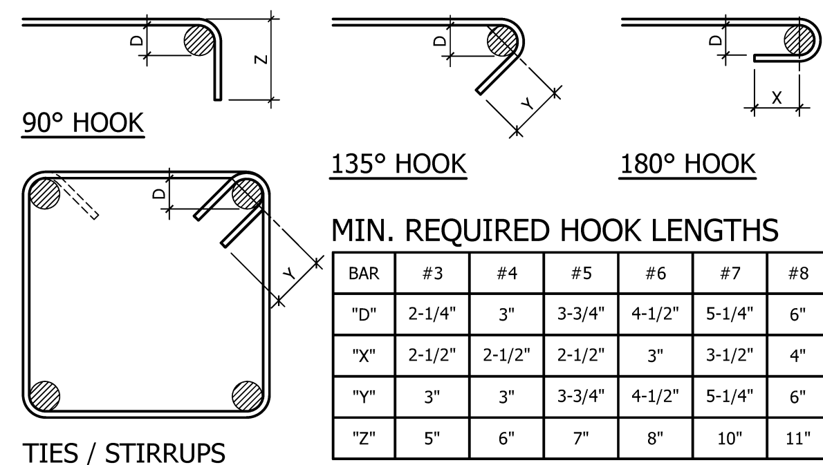
203 STD REINF. HOOKS - DOUBLE ROW
