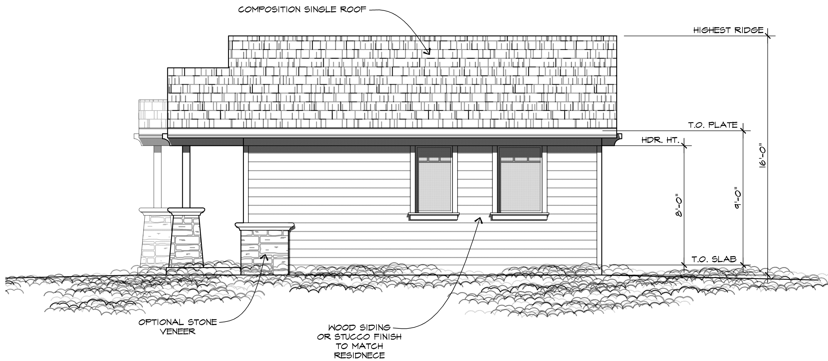
LEFT SIDE ELEVATION - (CRAFTSMAN STYLE)
