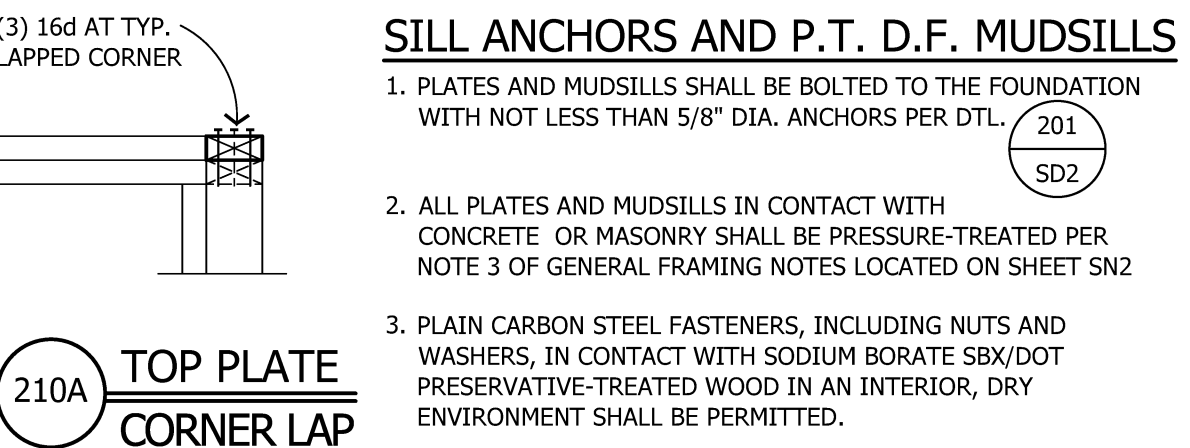
210A TOP PLATE CORNER LAP
