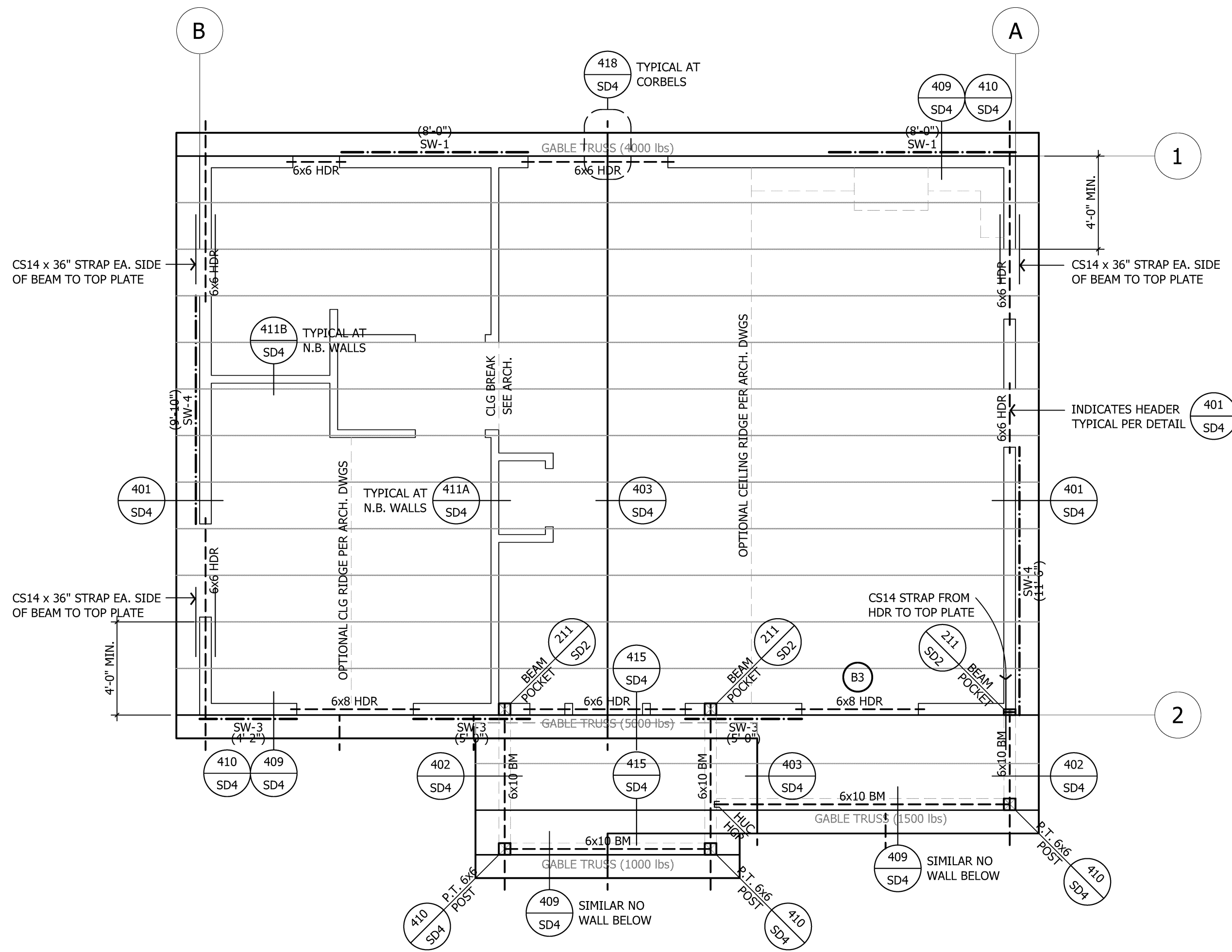
A ROOF FRAMING PLAN - CRAFTSMAN
