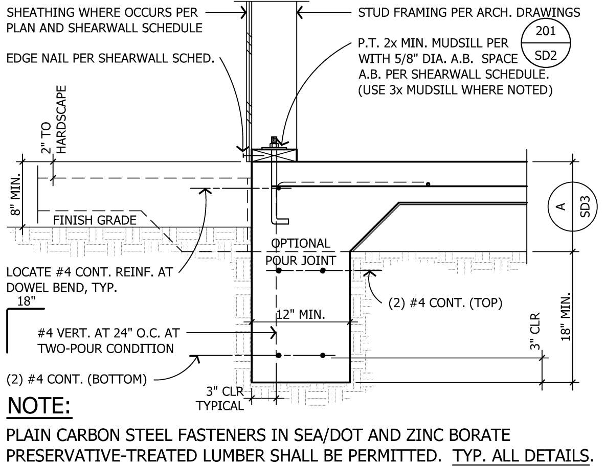
301 TYPICAL PERIMETER FOOTING
