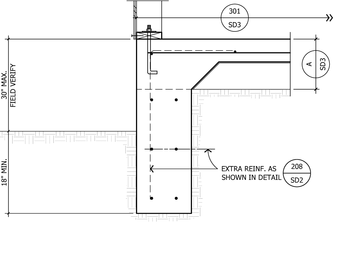
301B DEEPENED FOOTING AT LOW GRADE COND.
