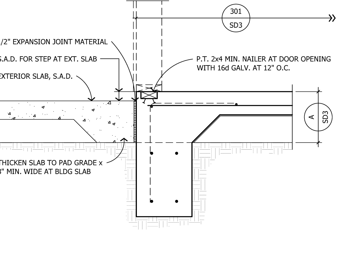
302 THRESHOLD EMBEDDED NAILER AT DOOR
