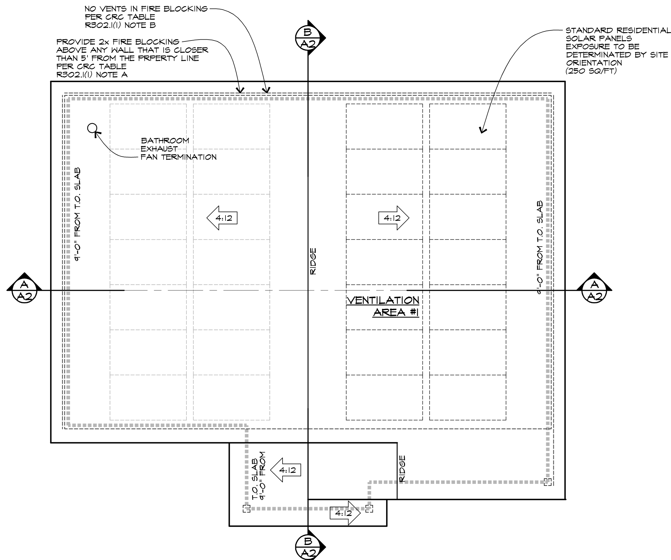
ROOF PLAN
