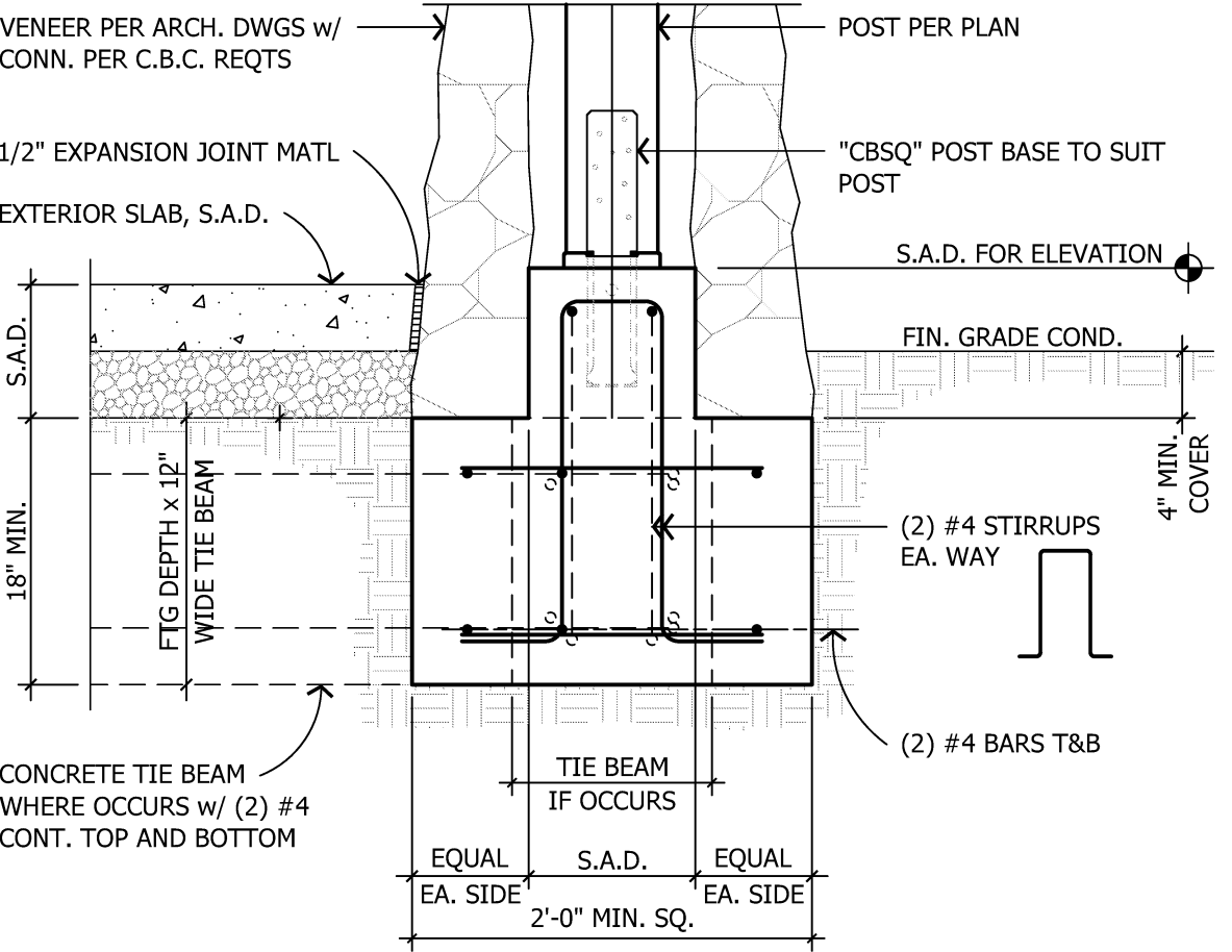
306 PORCH STUD COLUMN AND FOOTING
