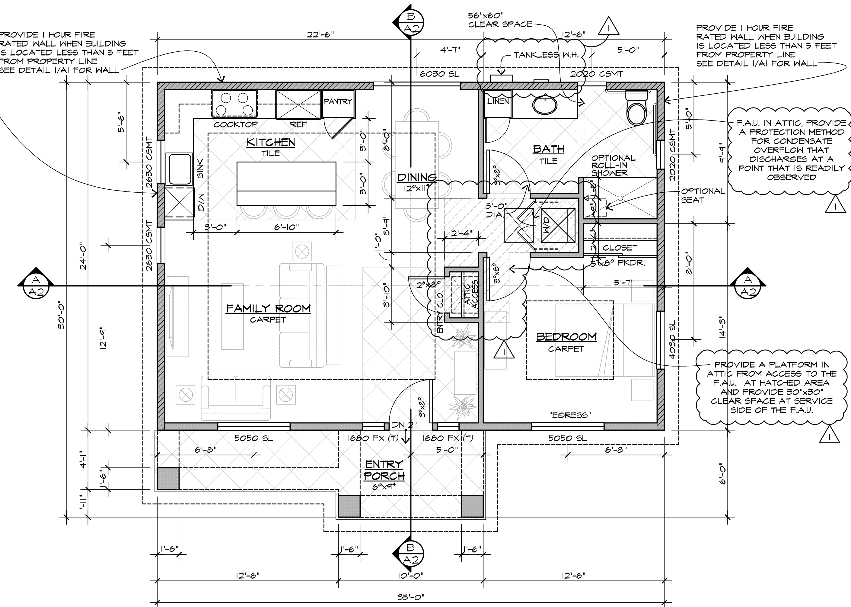
FLOOR PLAN (CONTEMPORARY STYLE)
