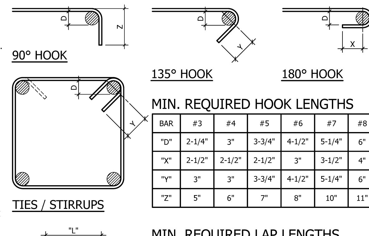
203 STD REINF. HOOKS - DOUBLE ROW
