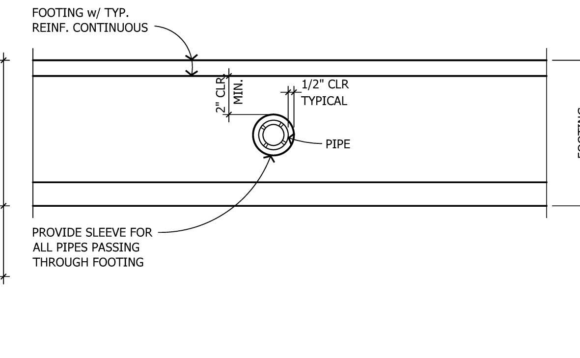
206D PIPE BETWEEN BARS
