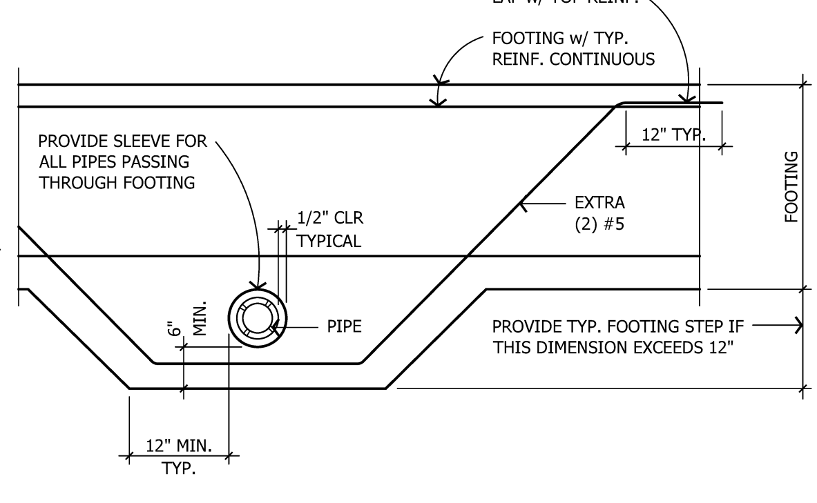
206A PIPE BELOW FOOTING
