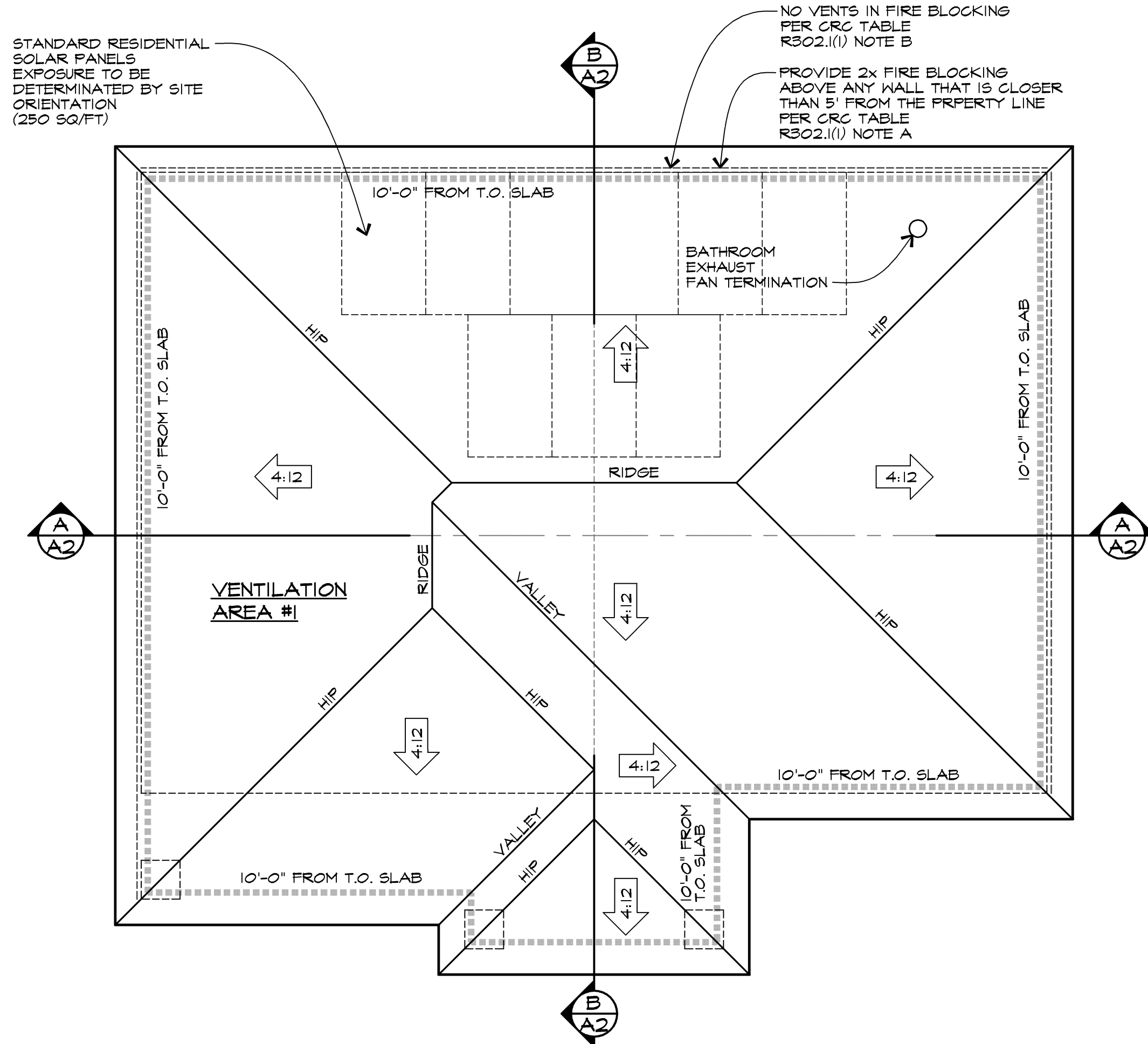
ROOF PLAN
