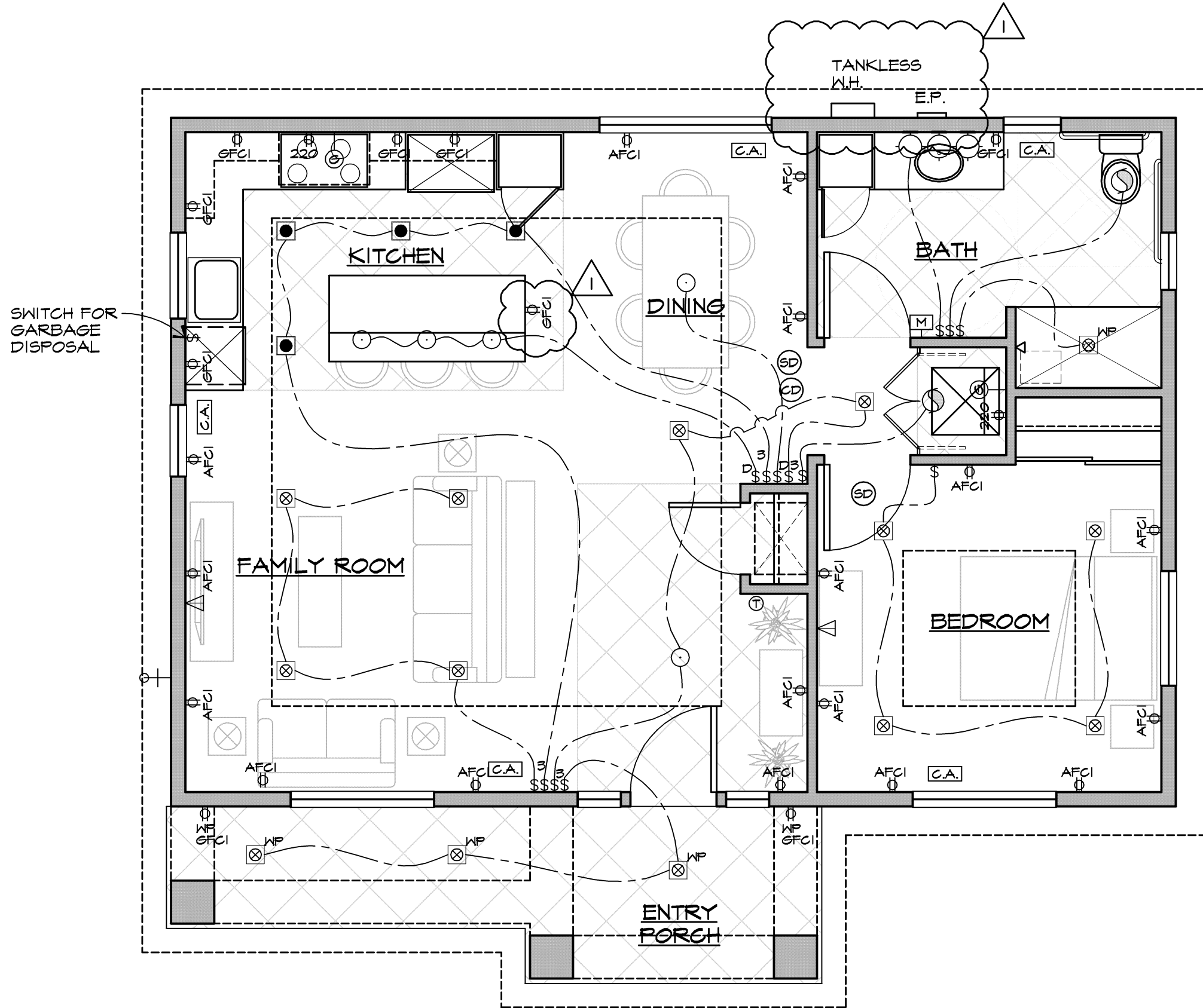
ELECTRICAL/ MECHANICAL FLOOR PLAN
