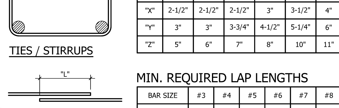
202B TYP. REINFORCING HOOKS AND LAPS
