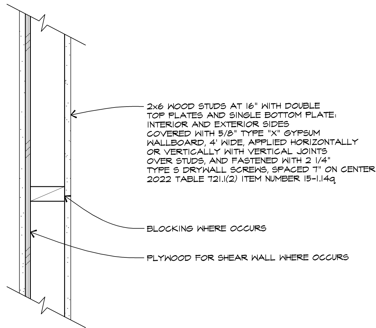
1 1 HOUR FIRE RATED WALL DETAIL A1
