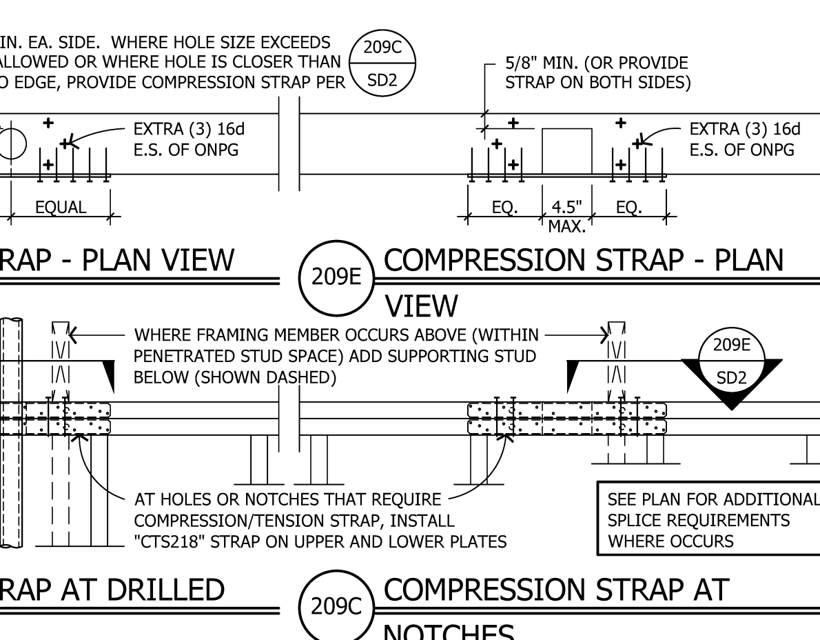
209C COMPRESSION STRAP AT NOTCHES
