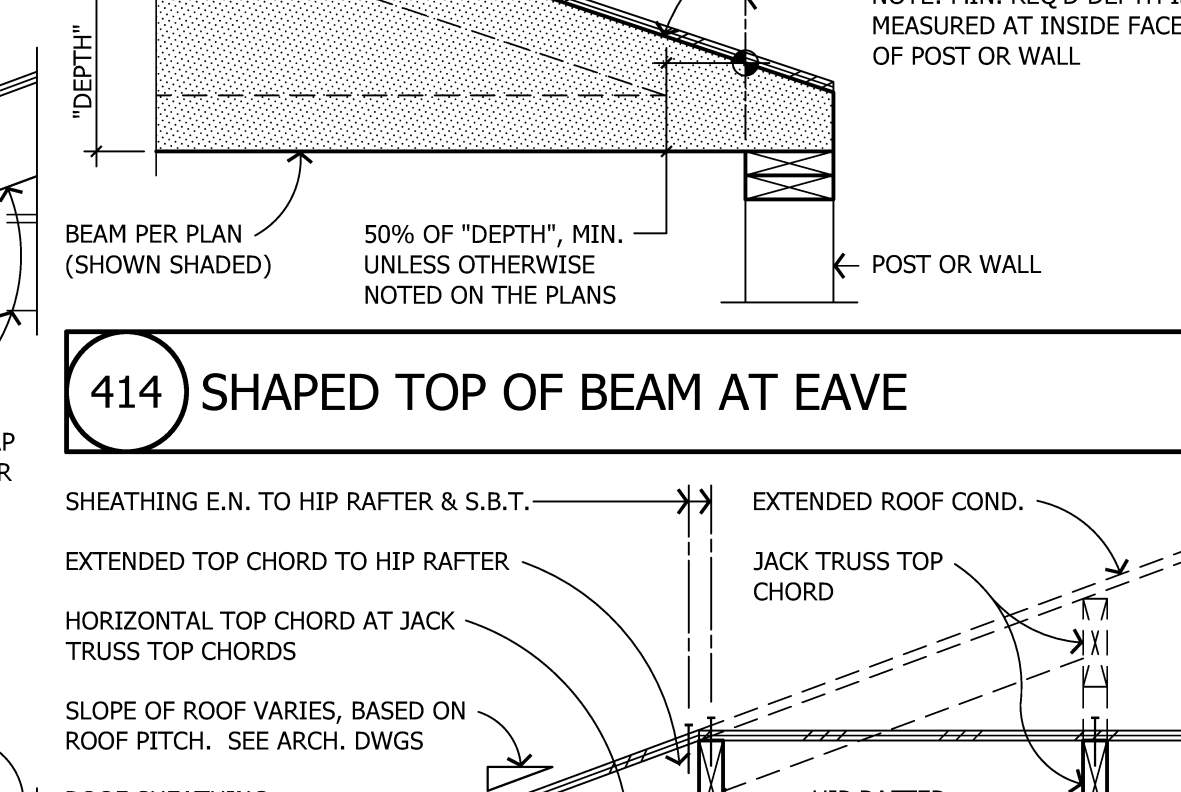
414 SHAPED TOP OF BEAM AT EAVE
