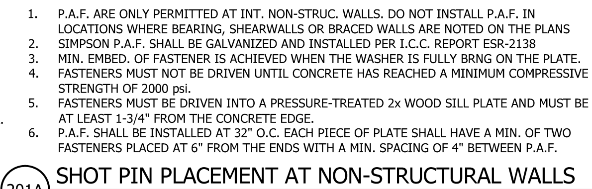
202A SHOT PIN PLACEMENT AT NON-STRUCTURAL WALLS
