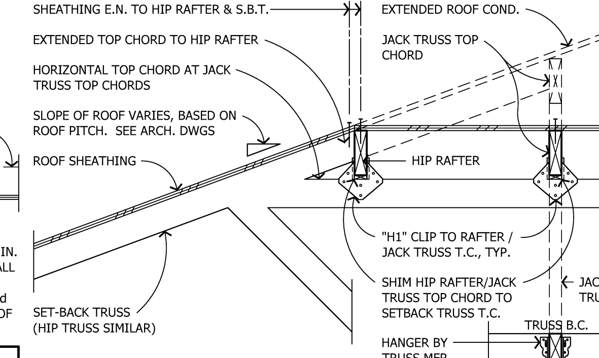
419 CONNECTION AT SET-BACK TRUSS
