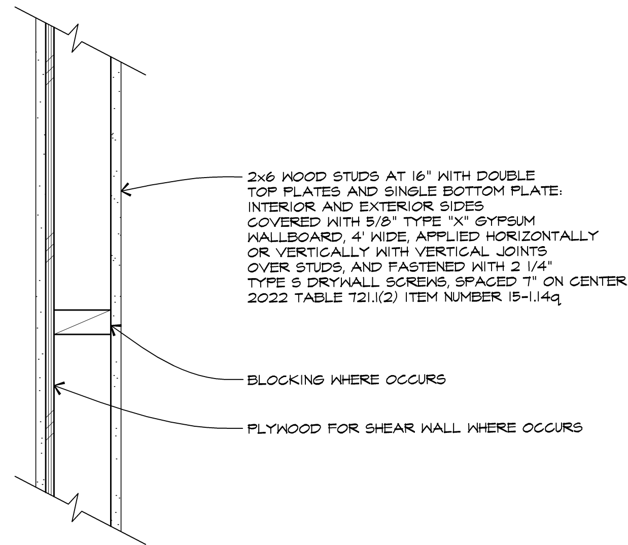
1 A1 1 HOUR FIRE RATED WALL DETAIL
