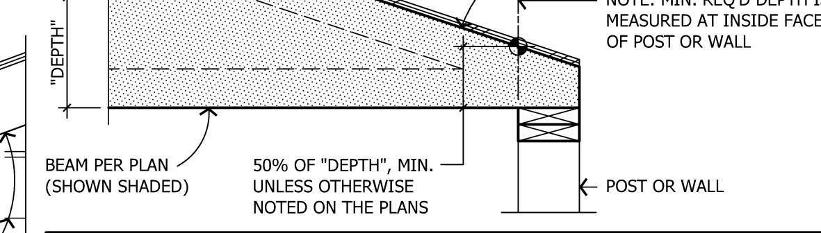
414 SHAPED TOP OF BEAM AT EAVE
