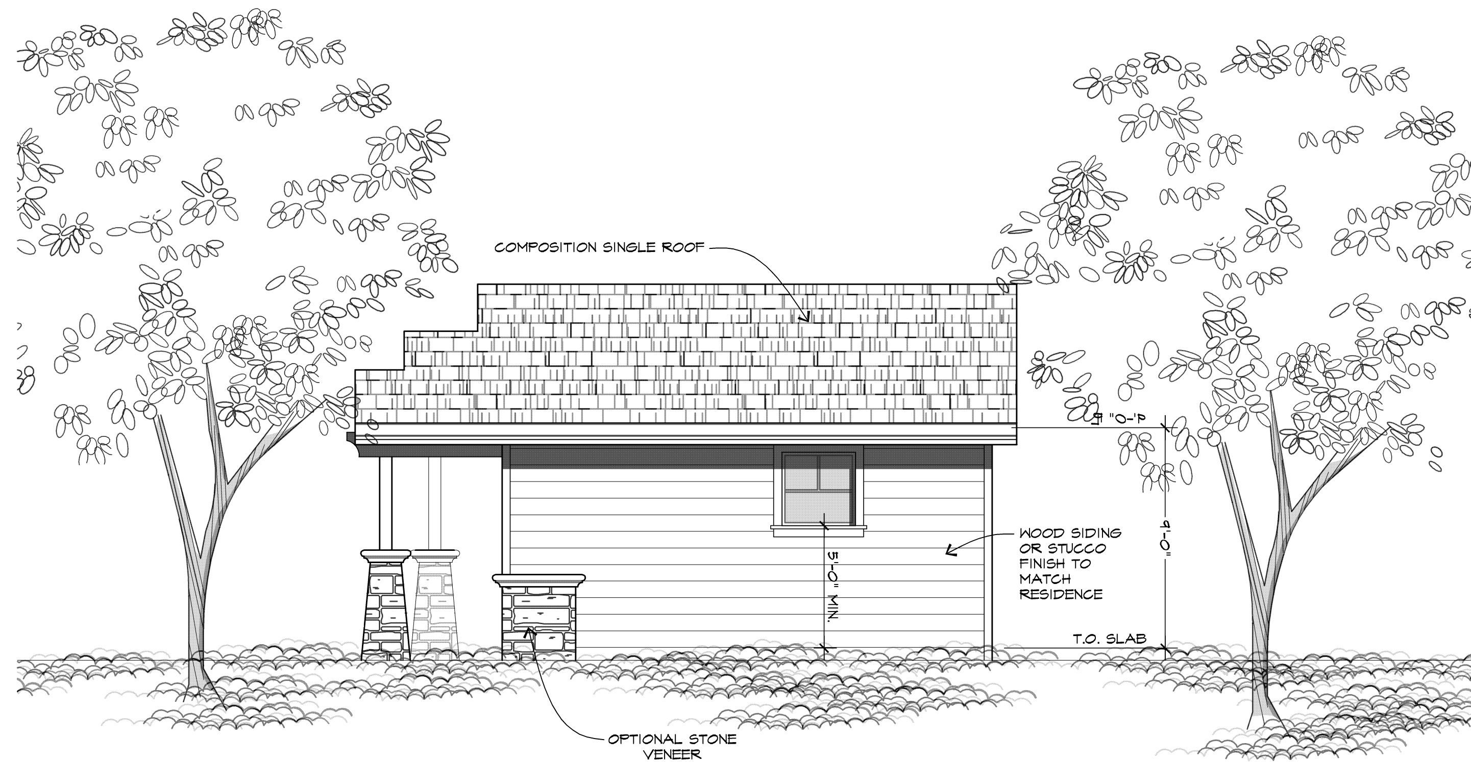
RIGHT ELEVATION (CRAFTSMAN STYLE)
