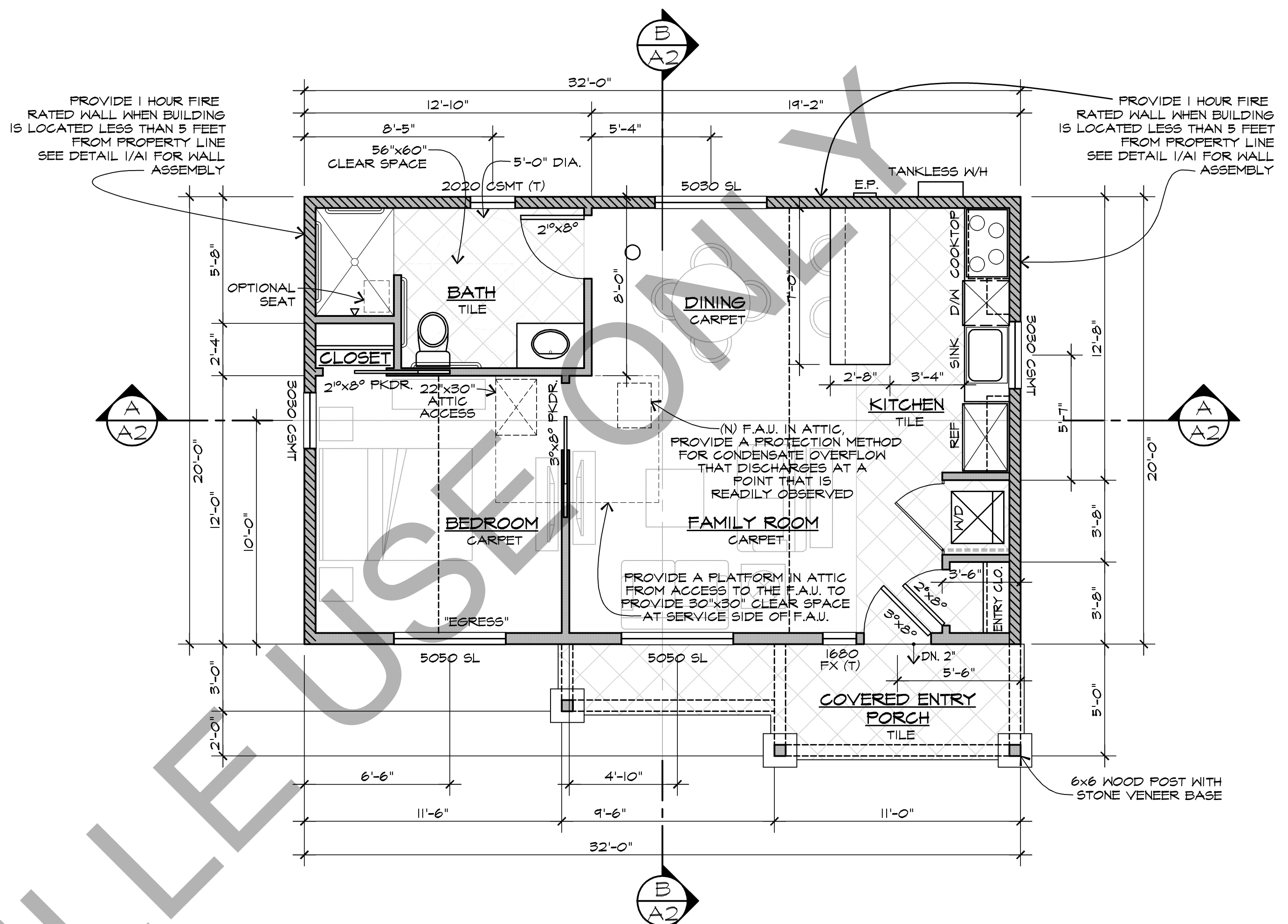
FLOOR PLAN (CRAFTSMAN STYLE)
