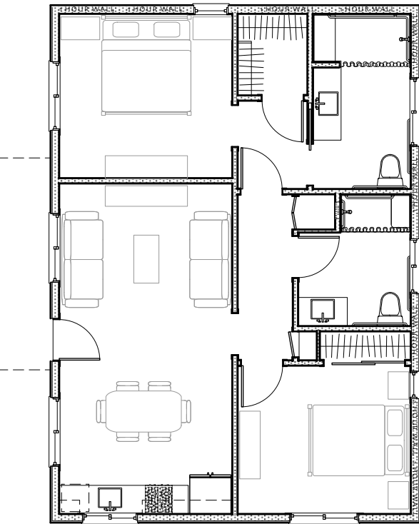
LEFT PLAN SCALE 1"=10'
