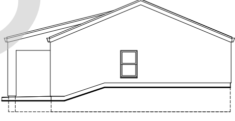
CRAFTSMAN RIGHT PLAN UPSLOPE LOT WITHOUT PIERS
