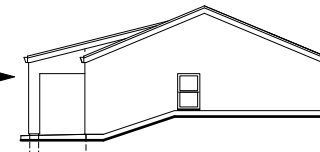
MEDITERRANEAN RIGHT PLAN UPSLOPE LOT WITHOUT PIERS
