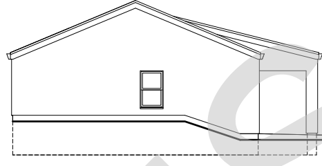
CONTEMPORARY LEFT PLAN UPSLOPE LOT
